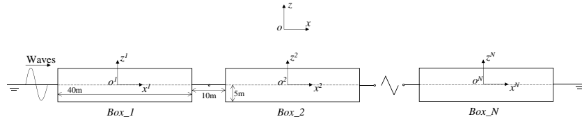
Figure 1: Configuration of N hinged boxes.
